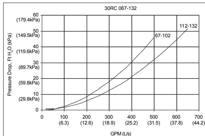
30RC 067-132 DX Evaporator Pressure Drop Curves
